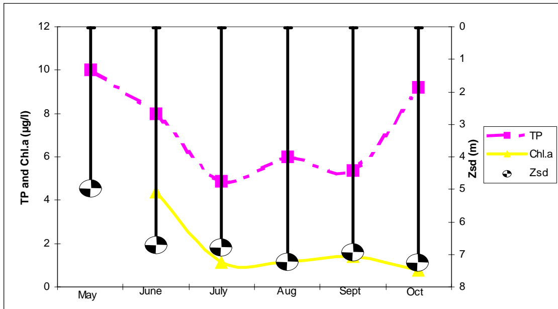
Figure 5- Eutrophication Data in a Typical (Monthly Mean) Year for Eagle Lake
