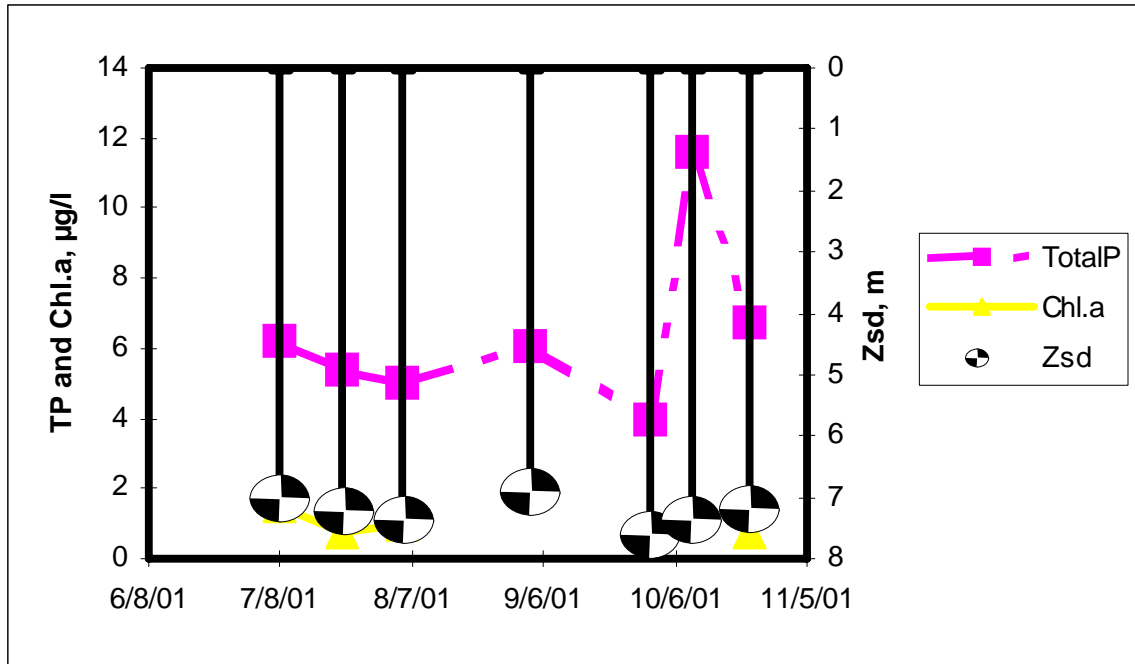
Figure 4. 2001 Eutrophication Data for Eagle Lake
