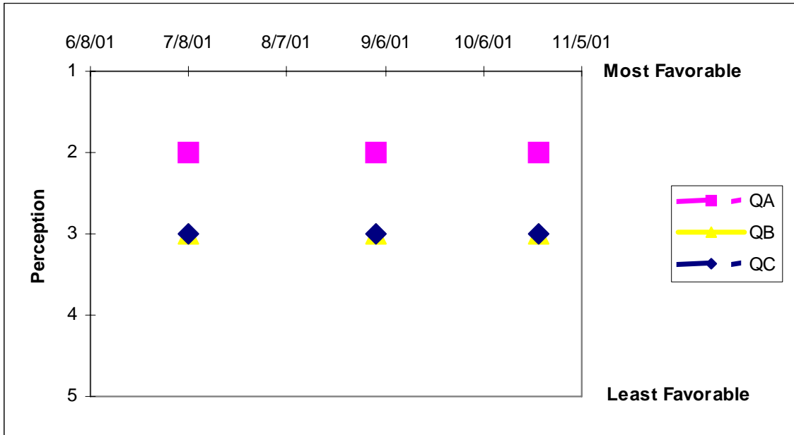
Figure 6. 2001 Lake Perception Data for Eagle Lake
